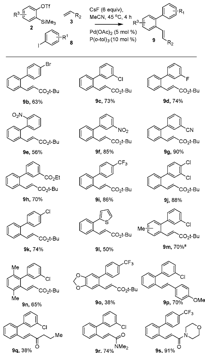
Scheme 2. 3CC of Aryl Iodides, Arynes and Heck Acceptors
