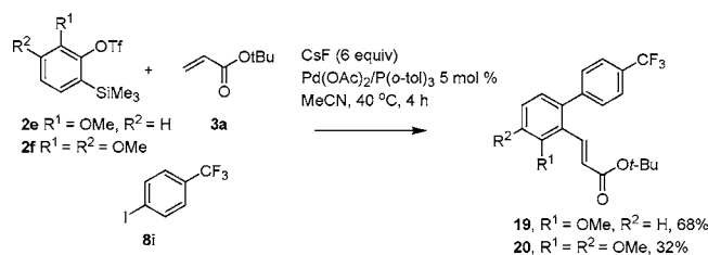
Scheme 5. 3CC of o -Methoxy-arynes
