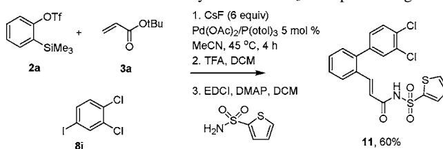
Scheme 3. 3CC for the Synthesis of EP 3 Receptor Antagonist
