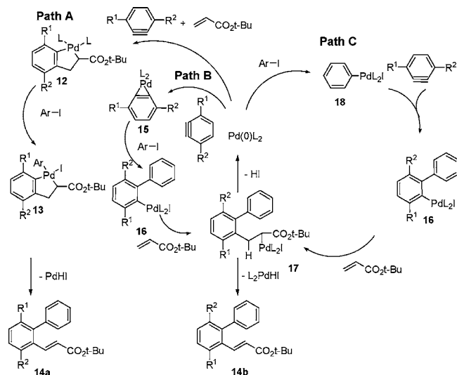
Scheme 4. Possible Three-Component Coupling Mechanisms
