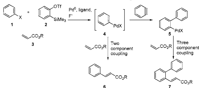
Scheme 1. Three-Component Coupling of Benzyne, Aryl Halide, and Heck Acceptor
